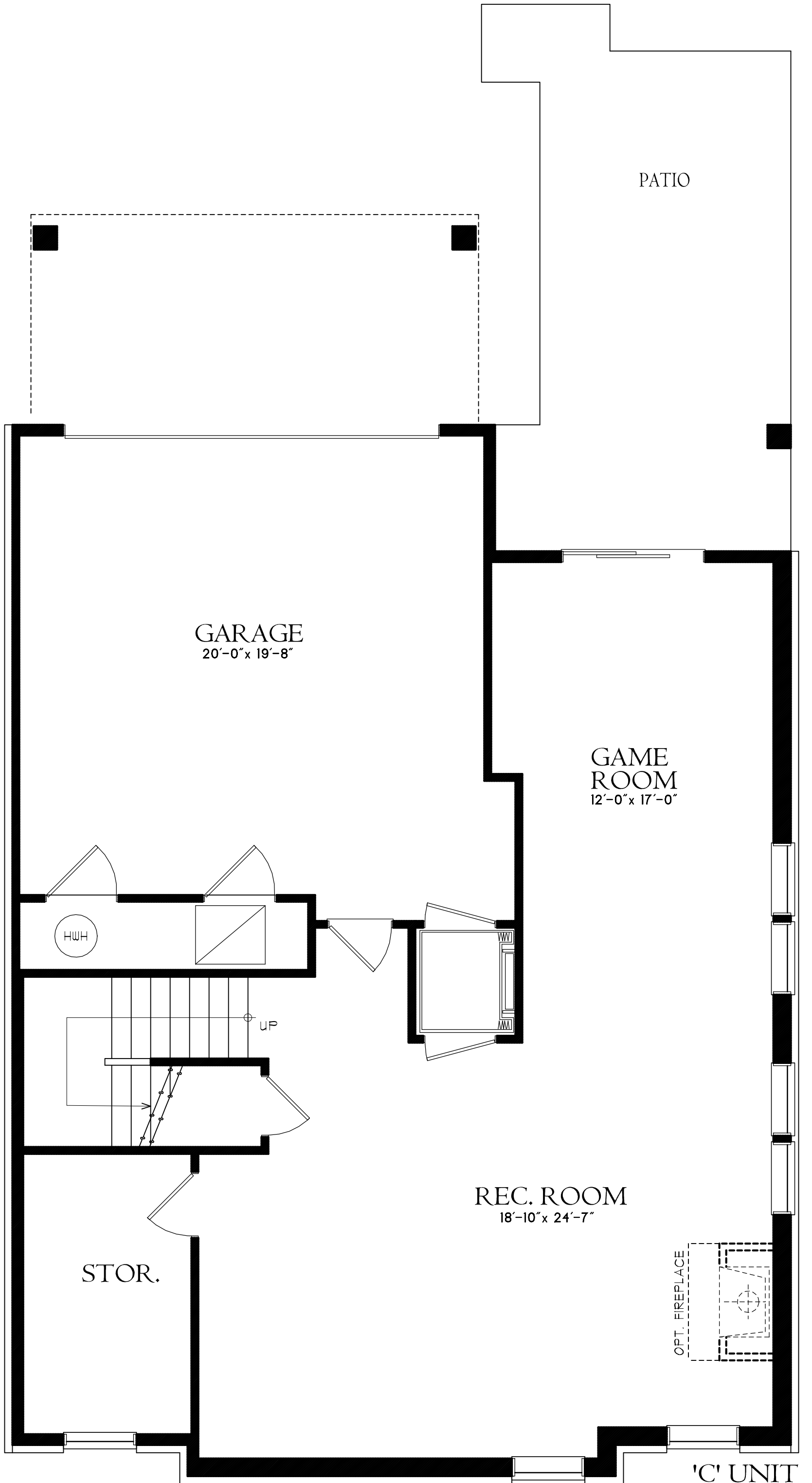
LOWER LEVEL PLAN WITH ELEVATOR OPTION
